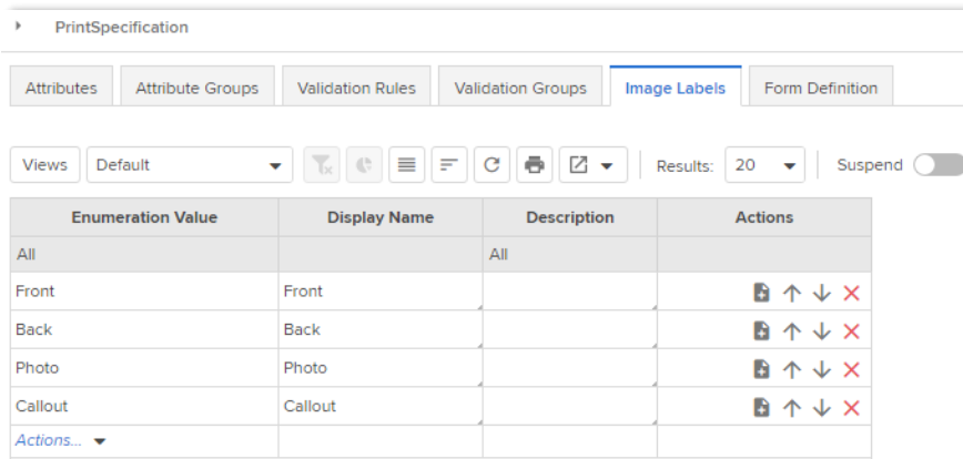
Figure 10: Defining Print Spec Labels on the Image Labels tab in C8
